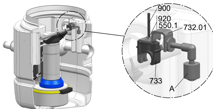
III. 6: Plan de montage, AmaDrainer 4.. SE, SD / 10, 35, AmaDrainer 5.. SE, SD / 10 K
