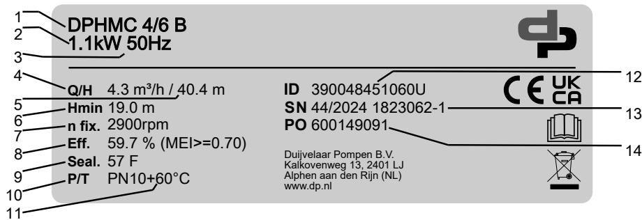
III. 2: Plaque signalétique (exemple)
